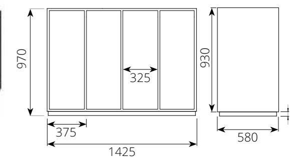
Quad Bay Single Door
